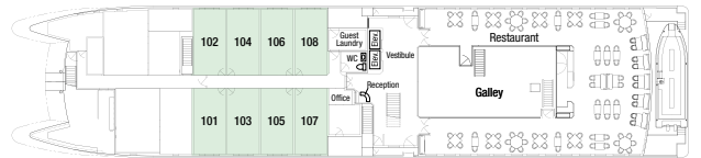
Main Deck
